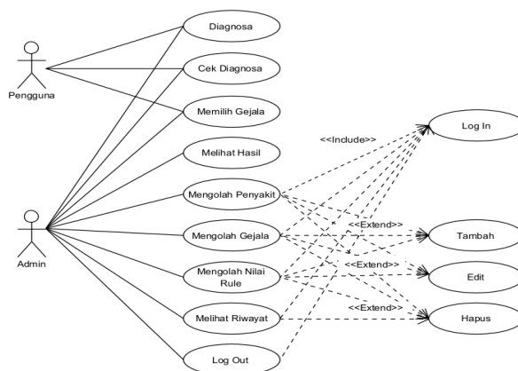
Gambar 2. Use Case
