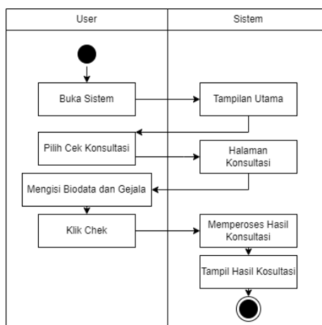
Gambar 3. Activity diagram
