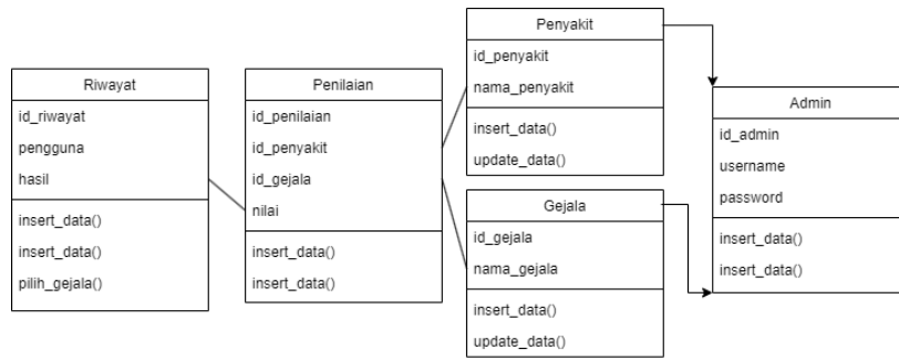
Gambar 4. Class diagram
